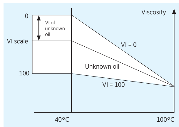
Figure 1: Schematic Representation of Viscosity Index
