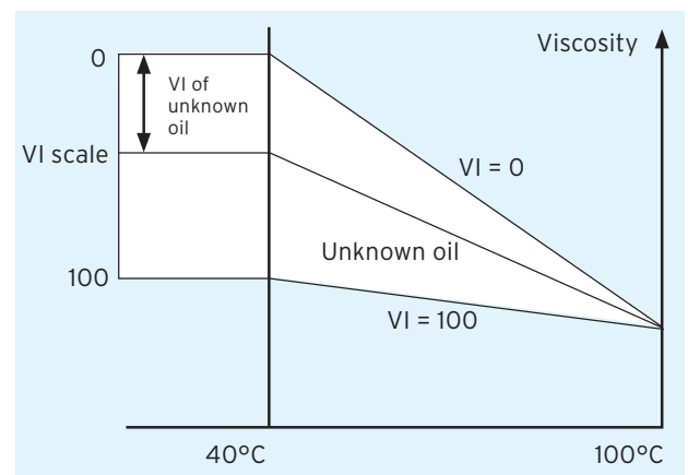
FIGURE 1: SCHEMATIC REPRESENTATION OF VISCOSITY INDEX
